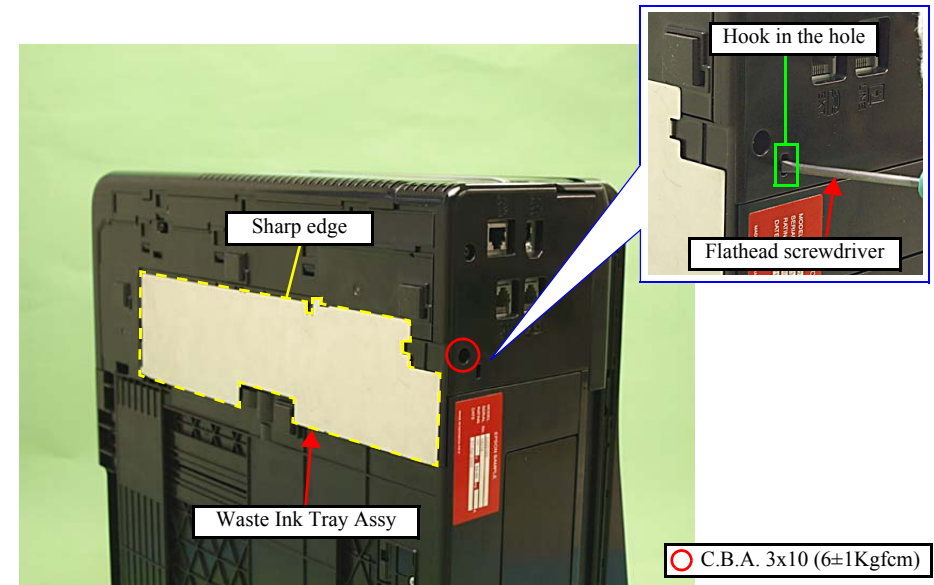
Figure 4-154. Removing the Waste Ink Tray Assy (1)
