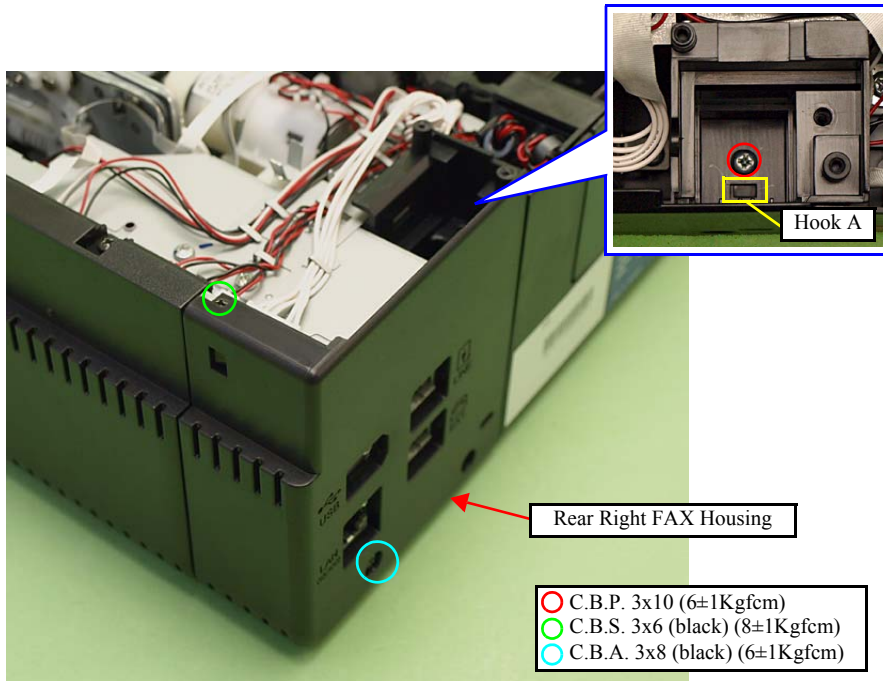
Figure 4-26. Removing the Rear Right FAX Housing (1)
