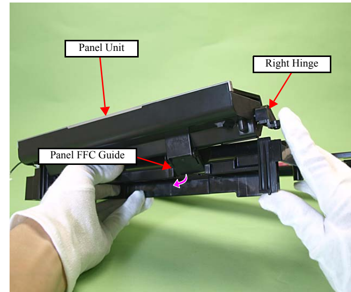
Figure 4-226. Removing the Panel Unit (1)
