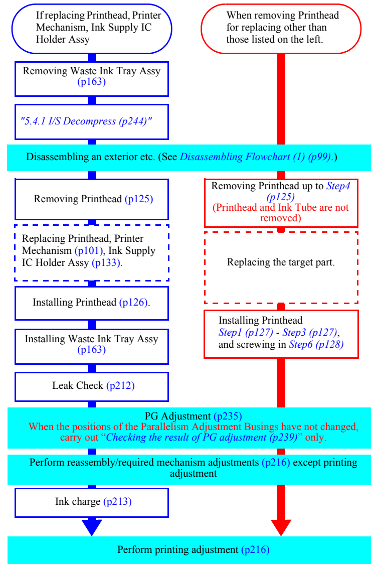
Figure 4-56. Related work for removing/installing the Printhead
