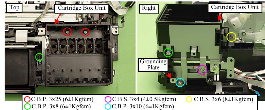
Figure 4-78. Removing the Cartridge Box Unit
