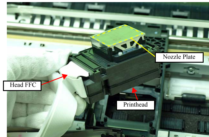
Figure 4-59. Removing the Printhead (2)
