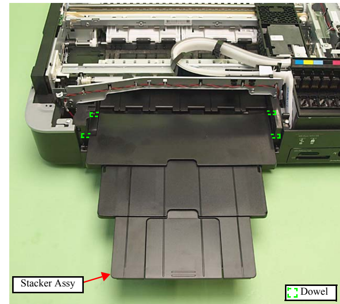
Figure 4-23. Removing the Stacker Assy
