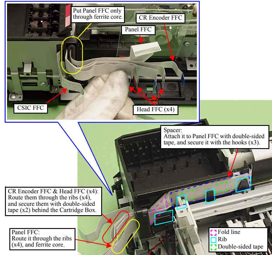
Figure 4-252. Routing to the FFC Holder (Artisan 700/PX700W/TX700W)
