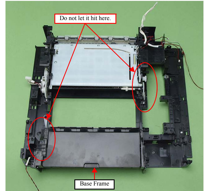
Figure 4-108. Installing the Main Frame
