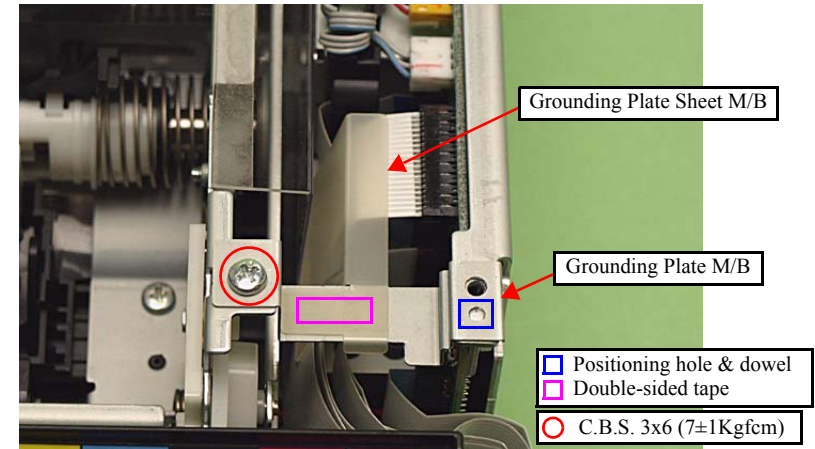
Figure 4-230. Removing the Grounding Plate M/B
