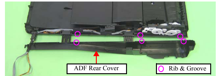
Figure 4-186. Installing the ADF Rear Cover
