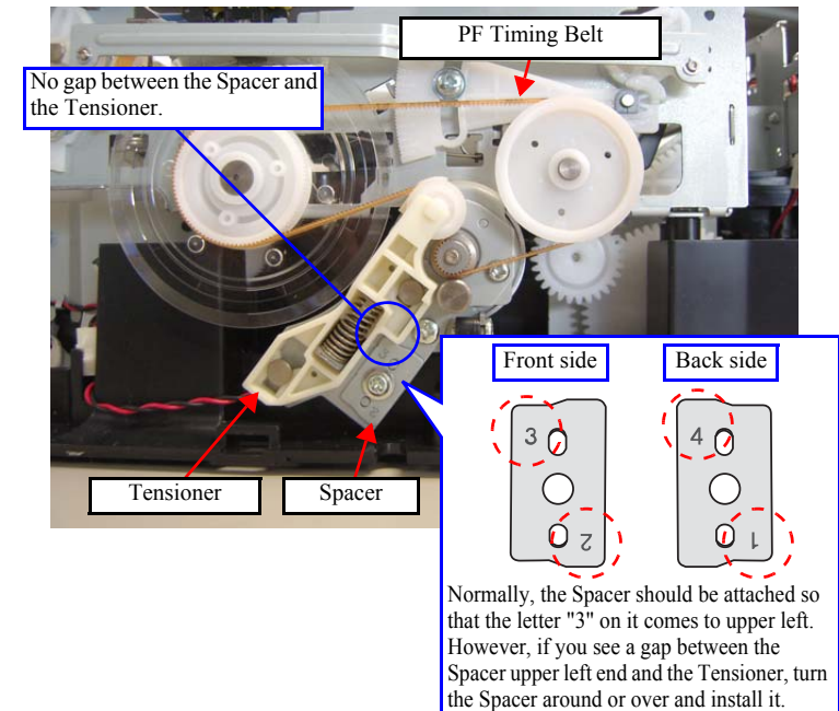
Figure 4-123. Installing the Spacer
