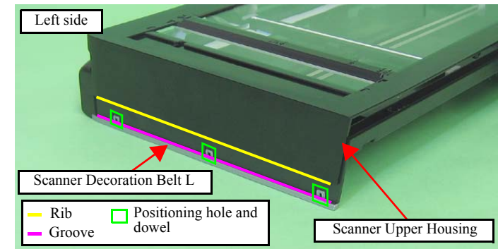
Figure 4-163. Installing the Scanner Upper Housing
