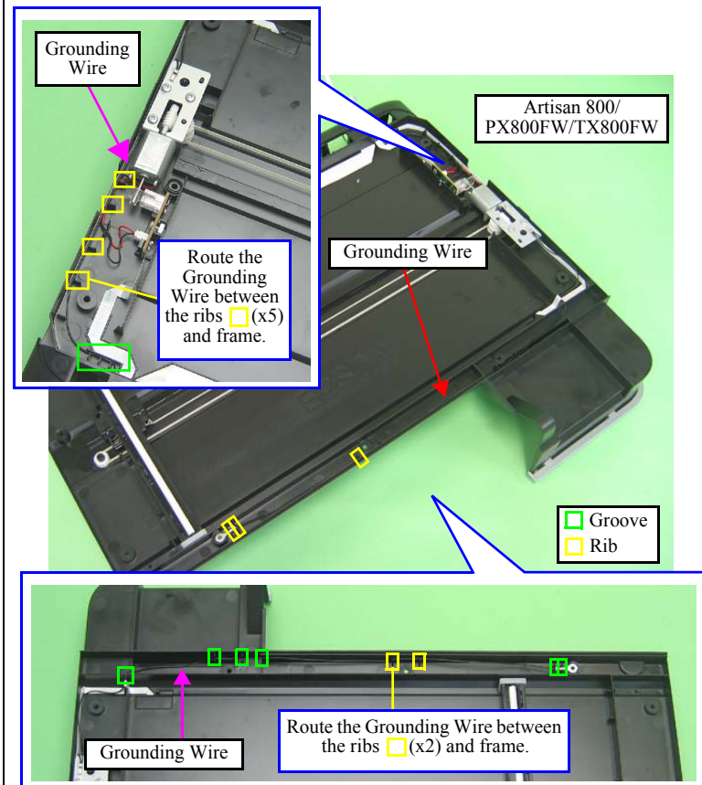
Figure 4-165. Routing the Grounding Wire (Artisan 800/PX800FW/TX800FW)
