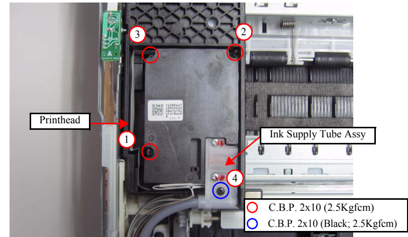
Figure 4-58. Removing the Printhead (1)
