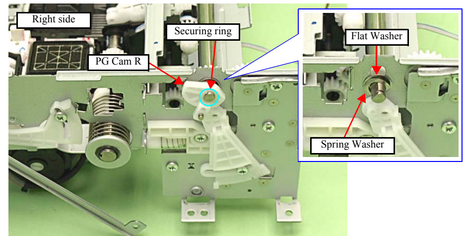
Figure 4-133. Removing the Carriage Unit (2)
