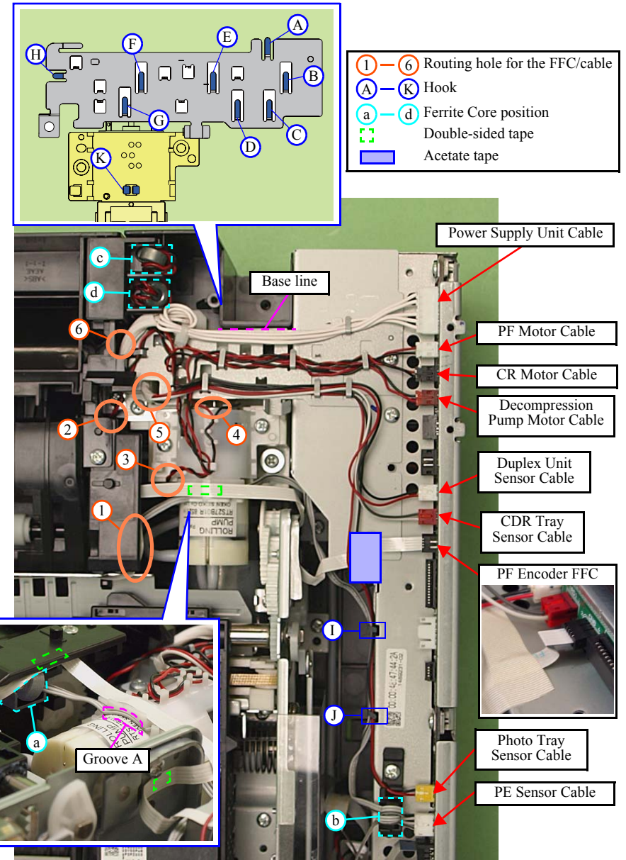
Figure 4-246. Main Board (Artisan 800/PX800FW/TX800FW)
