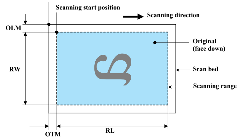
Figure 1-2. Scanning Range
