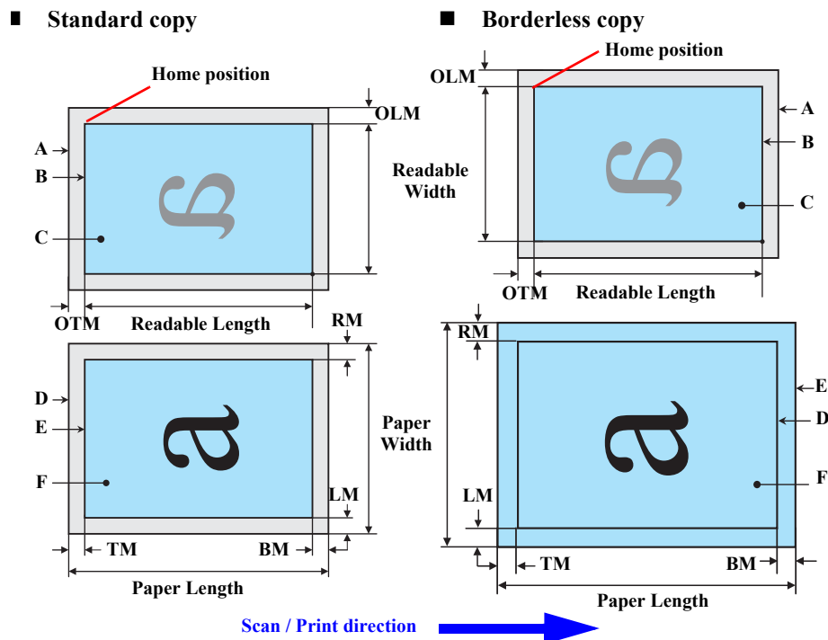
Figure 1-6. Relation Between Original and Copy (Borderless/With Borders)
