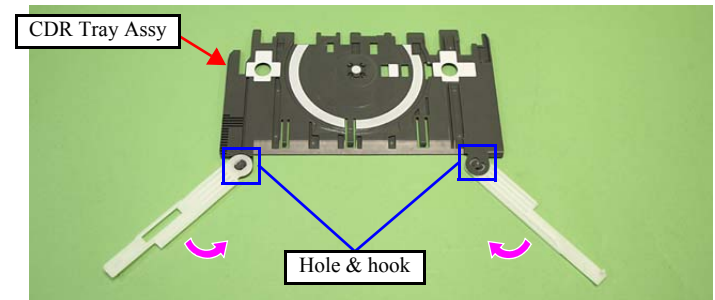
Figure 4-96. Reassembling the CDR Tray Assy
