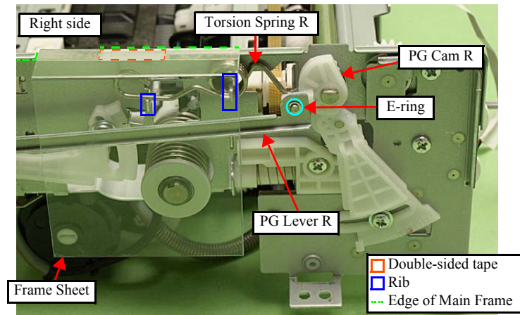
Figure 4-132. Removing the Carriage Unit (1)
