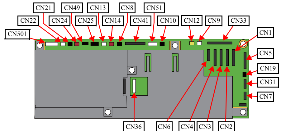
Figure 4-39. Connector position on the Main Board
