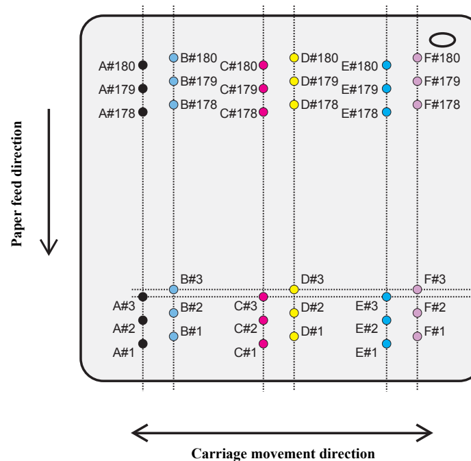
Figure 2-2. Nozzle Layout
