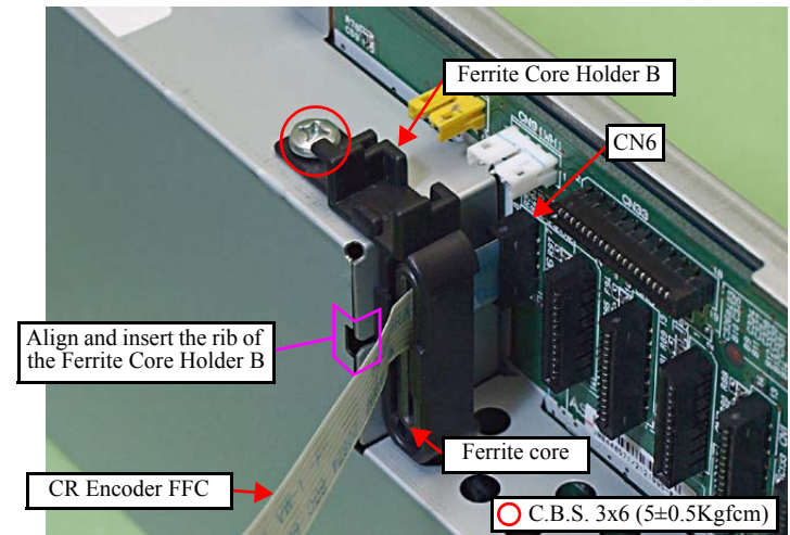
Figure 4-236. Attaching the CR Encoder FFC
