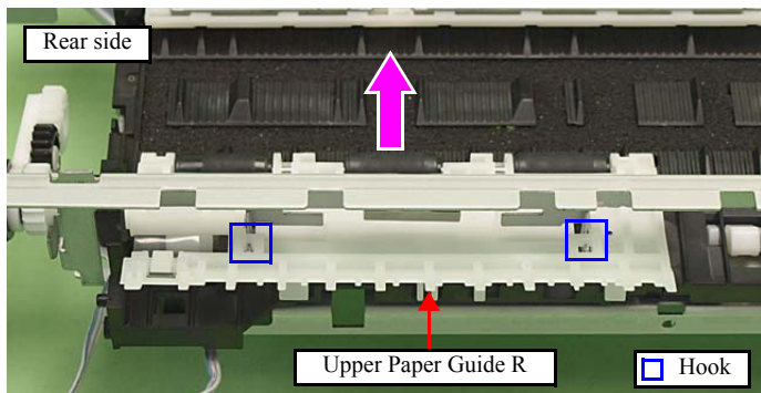
Figure 4-150. Removing the Upper Paper Guide R
