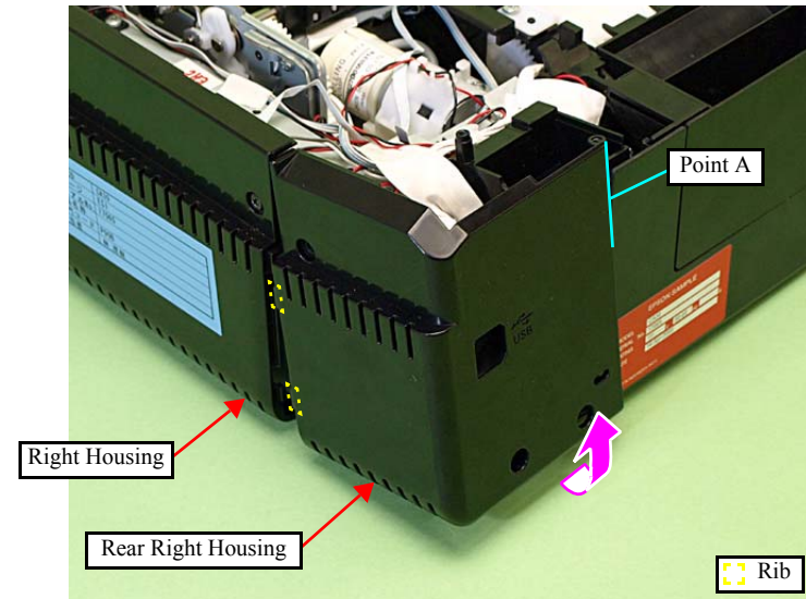
Figure 4-221. Removing the Rear Right Housing (2)
