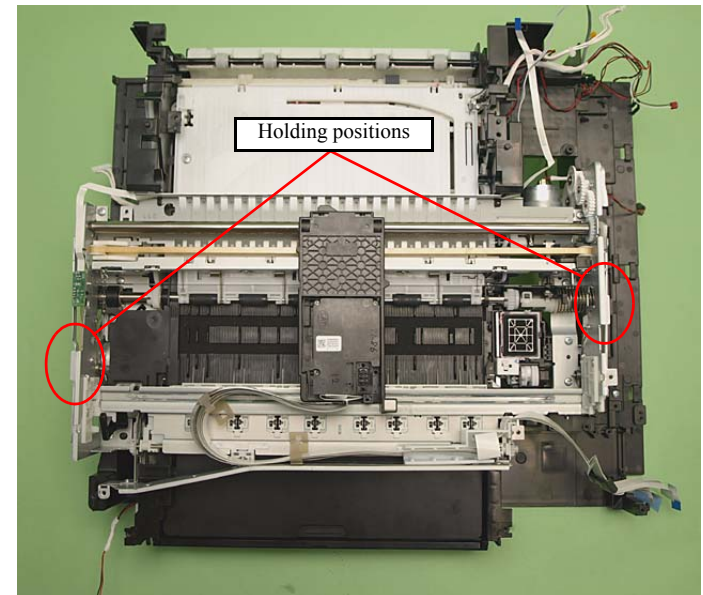
Figure 4-104. Holding positions of Main Frame
