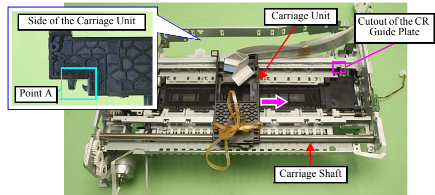
Figure 4-136. Removing the Carriage Unit (5)
