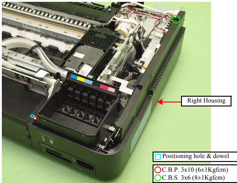
Figure 4-28. Removing the Right Housing/Card Cover (1)
