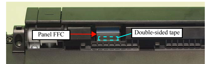
Figure 4-215. Installing the Upper Housing
