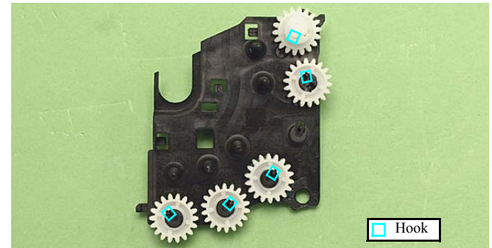
Figure 4-141. Installing the Transmission Holder Assy (1)
