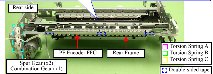
Figure 4-144. Removing the Rear Frame (1)
