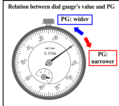
Figure 5-38. PG adjustment
