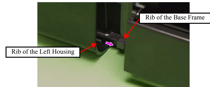
Figure 4-219. Installing the Left Housing
