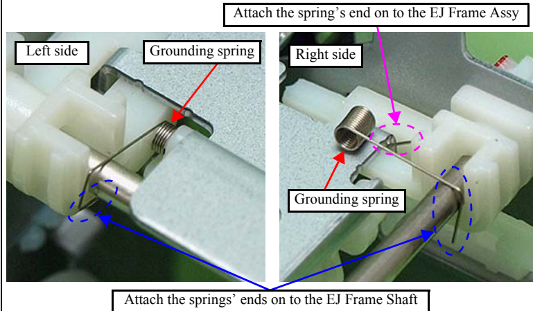
Figure 4-114. Attaching the grounding spring
