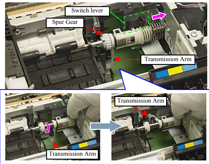
Figure 4-86. Installing the Ink System (2)
