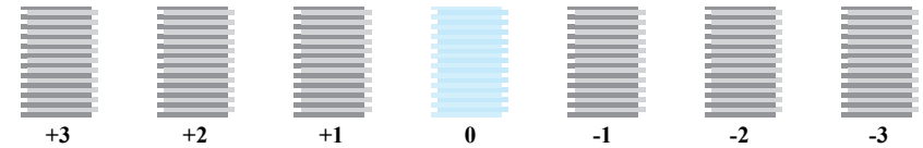
Figure 5-5. Head angular adjustment Pattern Printing (2)
