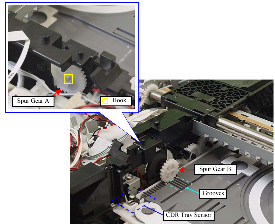
Figure 4-94. Removing the CDR Tray Assy (1)
