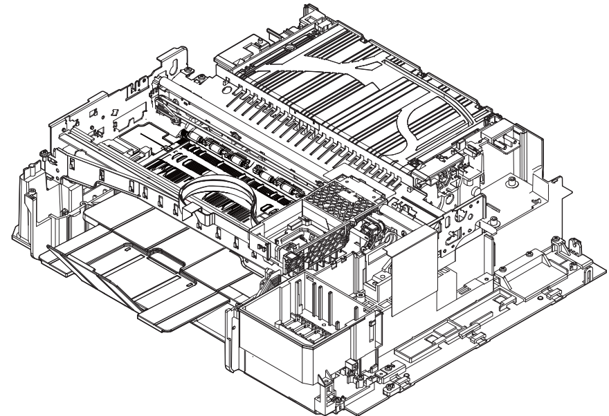
Figure 4-1. Printer Mechanism
