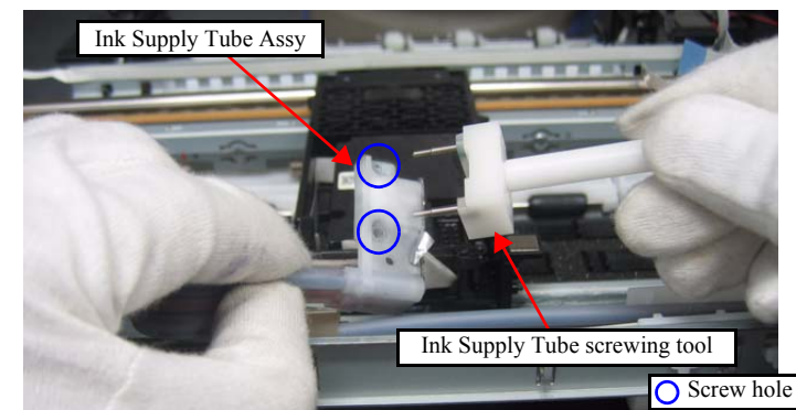
Figure 4-65. Assembling the Printhead (2)
