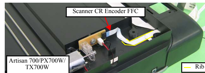
Figure 4-173. Routing the FFC (Artisan 700/PX700W/TX700W)
