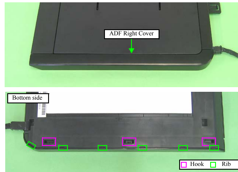
Figure 4-183. Removing the ADF Right Cover
