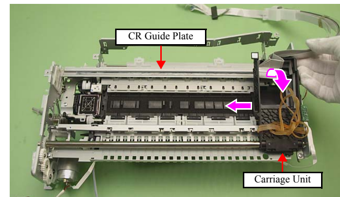
Figure 4-137. Removing the Carriage Unit (6)
