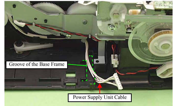
Figure 4-50. Installing the Power Supply Unit
