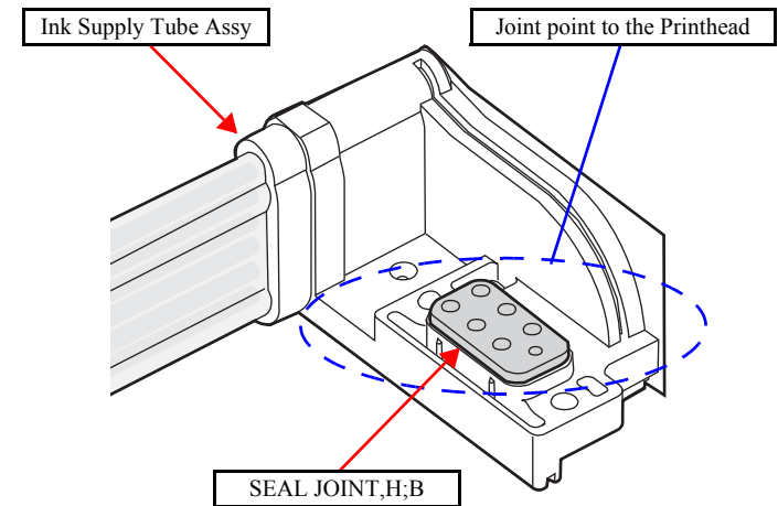
Figure 4-64. SEAL JOINT,H;B
