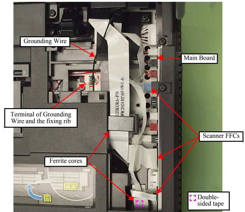
Figure 4-6. Removing the Scanner Unit (1)
