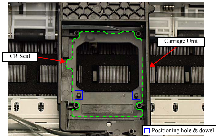
Figure 4-62. Installing the CR Seal
