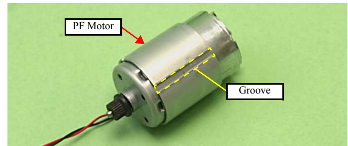
Figure 4-122. Installing the PF Motor
