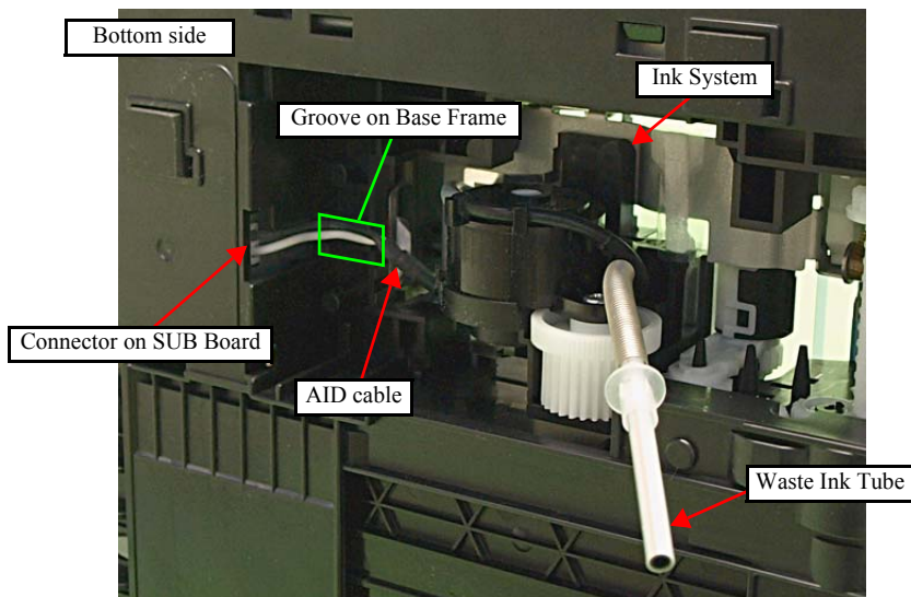
Figure 4-84. Removing the Ink System (2)
