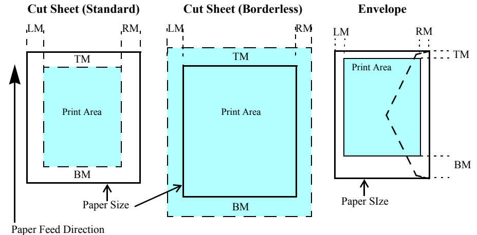
Figure 1-1. Printing Area
