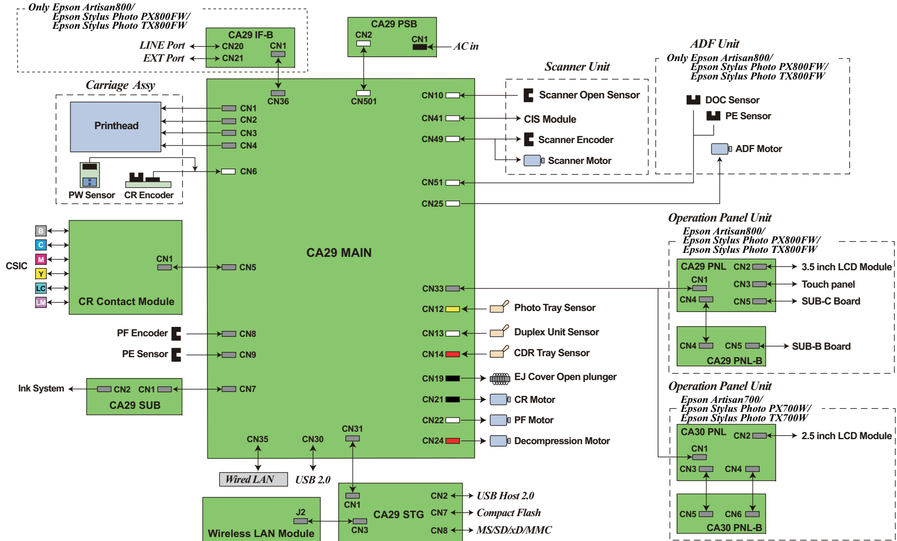
Figure 7-1. Block Diagram
