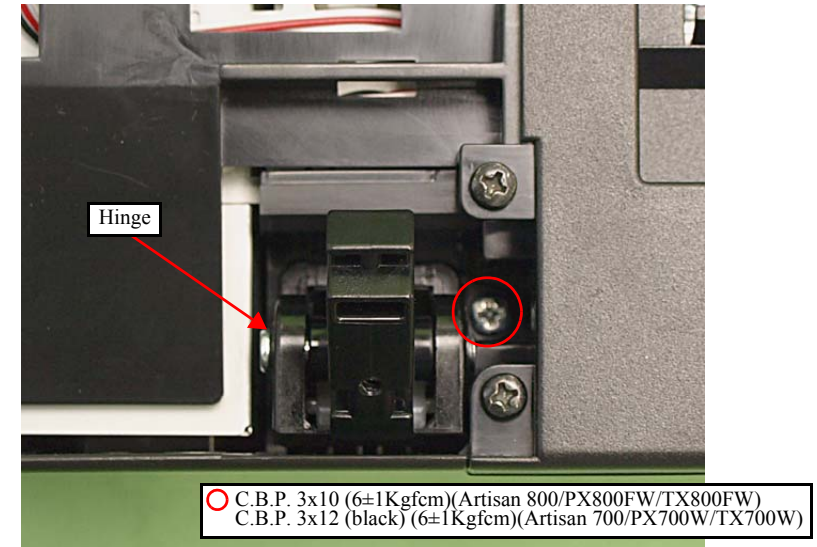
Figure 4-12. Removing the Hinge
