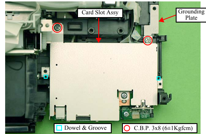
Figure 4-238. Removing the Card Slot Assy (1)
