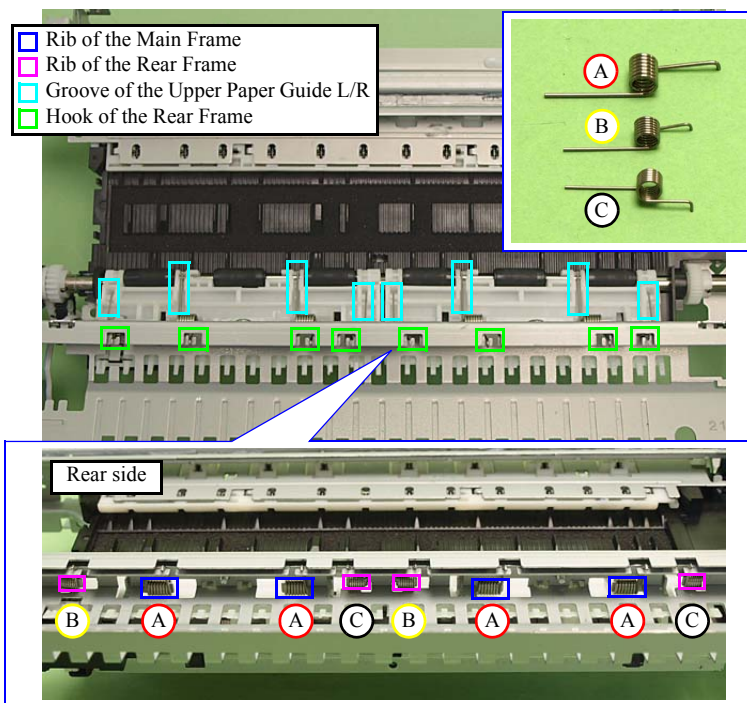
Figure 4-146. Attaching the Torsion Spring
