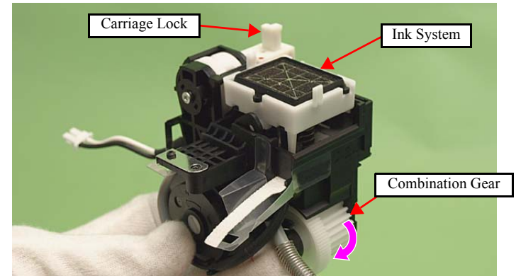
Figure 4-85. Installing the Ink System (1)
