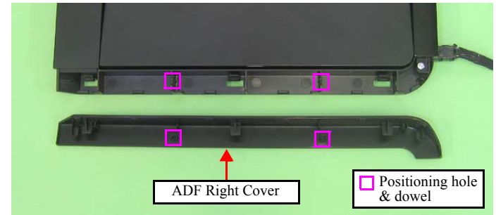
Figure 4-185. Installing the ADF Right Cover
