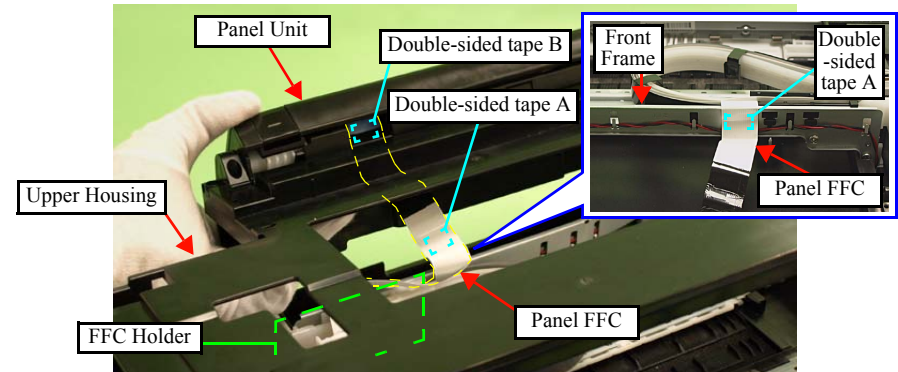
Figure 4-214. Removing the Upper Housing (4)
