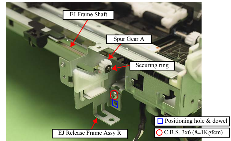
Figure 4-110. Removing the EJ Release Frame Assy R
