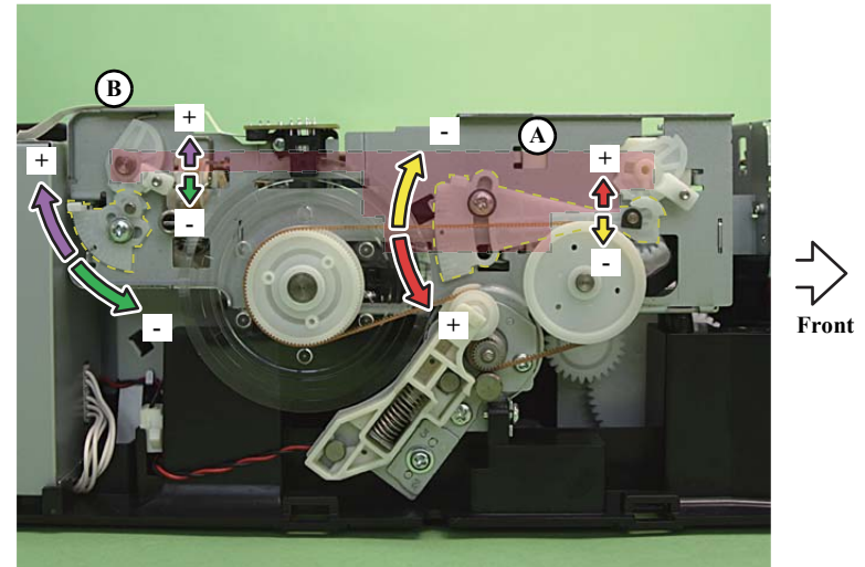
Figure 5-39. Operating the parallelism adjustment bushing (Left side)
