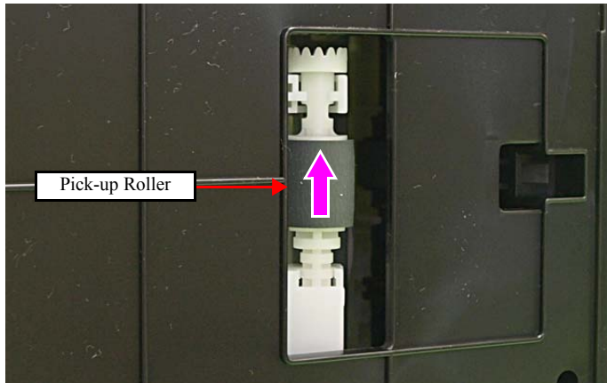
Figure 4-103. Removing the Pick-up Roller (2)
