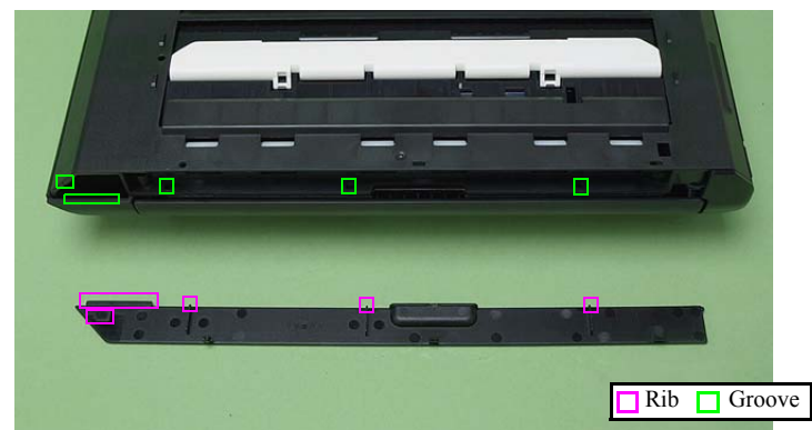
Figure 4-181. Installing the ADF Cover L
