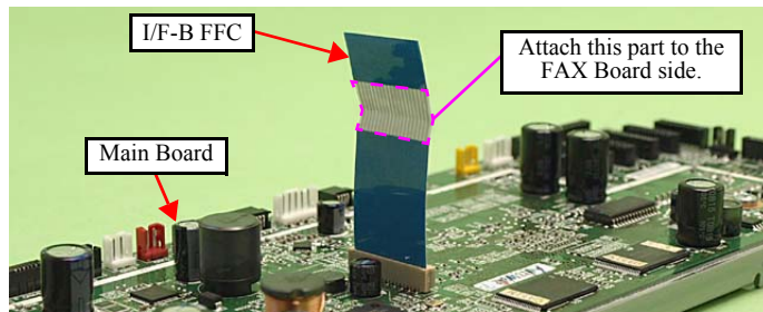
Figure 4-45. Connecting the I/F-B FFC
