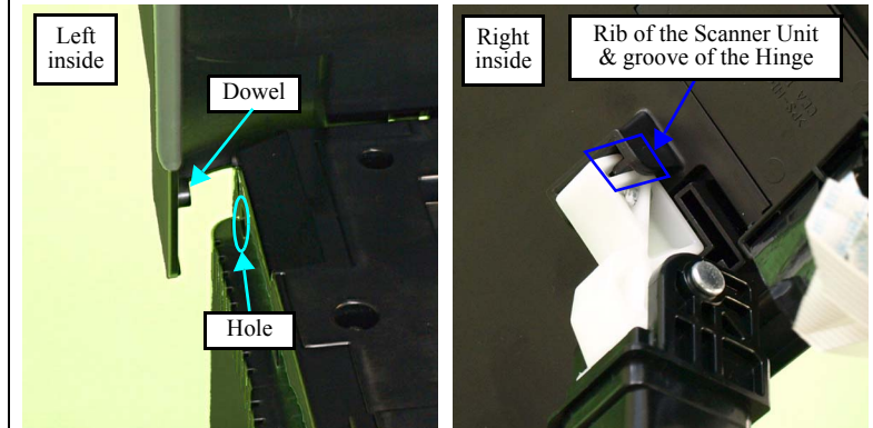
Figure 4-207. Installing the Scanner Unit (1)
