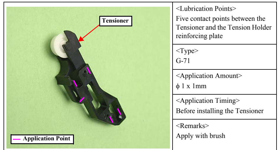
Figure 6-16. Lubrication of the Tensioner
