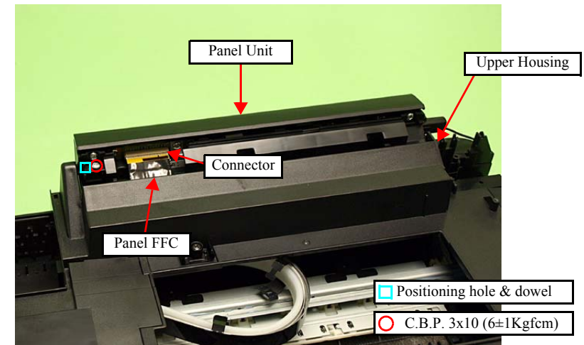
Figure 4-38. Removing the Panel Unit (2)
