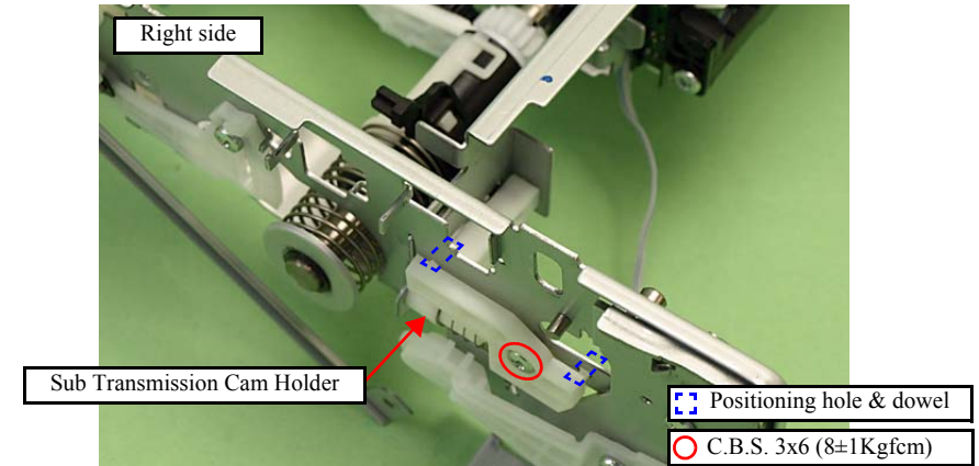
Figure 4-148. Removing the Upper Paper Guide R/PE Sensor
