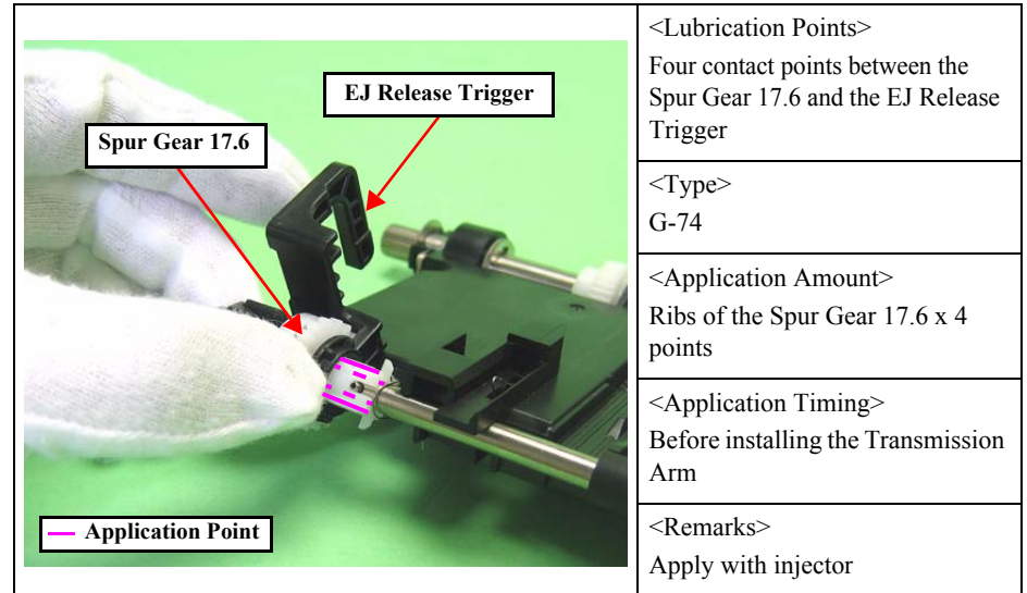
Figure 6-15. Lubrication of the Spur Gear 17.6
