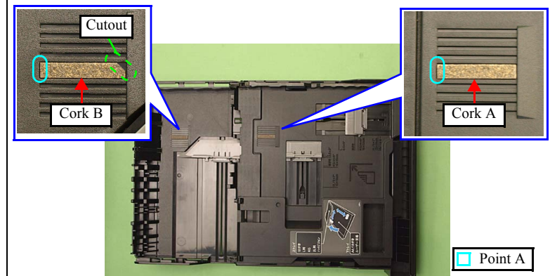
Figure 4-33. Attaching the cork
