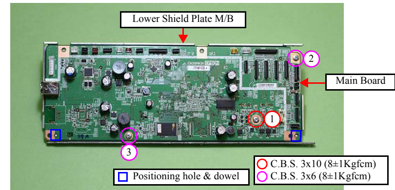
Figure 4-234. Removing the Main Board (3)
