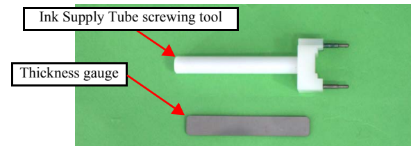
Figure 4-61. Ink Supply Tube screwing tool
