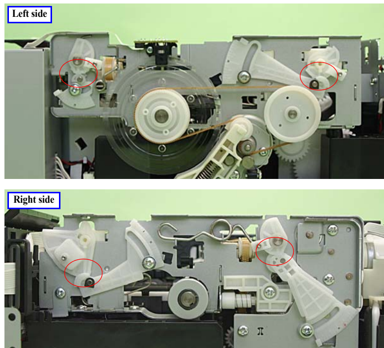
Figure 5-36. PG position when adjusting
