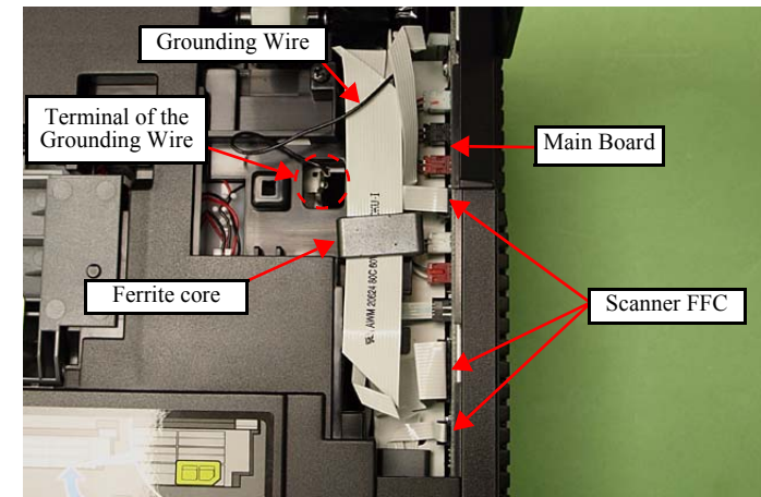
Figure 4-204. Removing the Scanner Unit (1)
