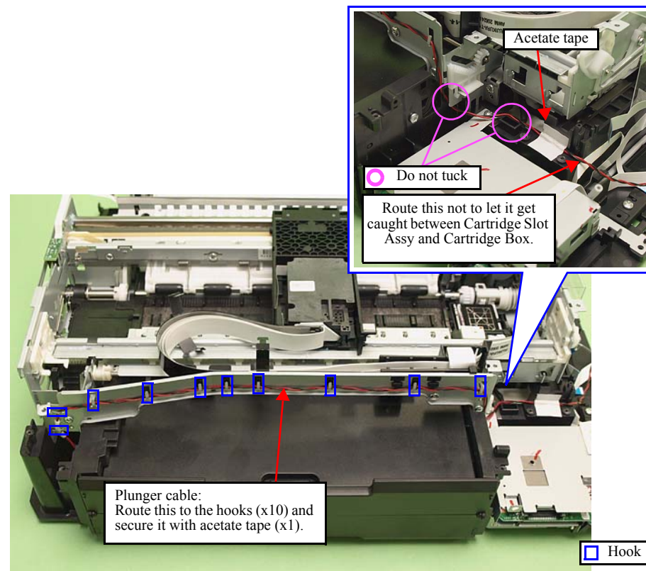
Figure 4-254. Plunger Cable
